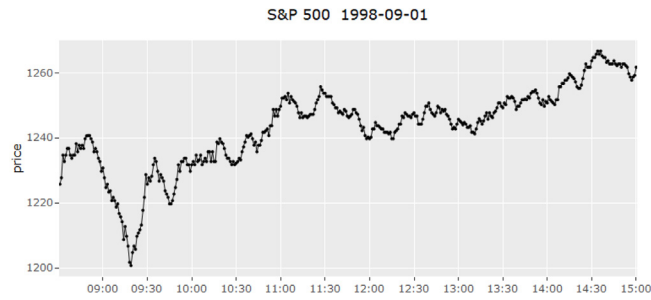
Fig. 1. S&P 500 index futures values on September 1, 1998.
