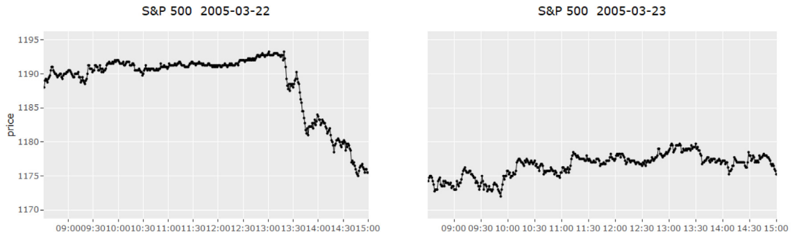
Fig. 2. E-mini S&P 500 index futures price on March 22 and 23, 2005.
