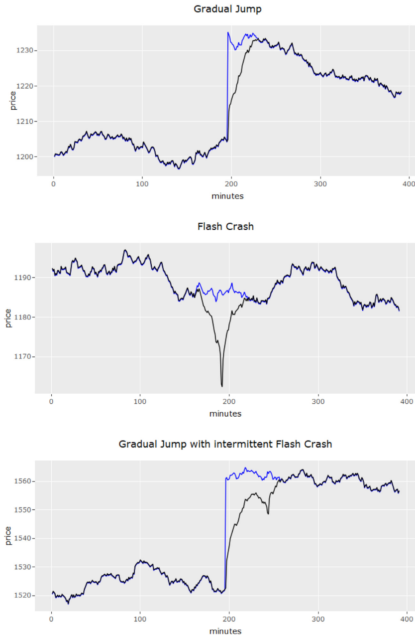
Fig. 3. Simulated price paths of the persistent noise model (6) in Assumption 3 for a gradual jump, flash crash, and gradual jump with an intermittent flash crash. Section 4.1 provides detailed specifications of these cases. The efficient price, \exp(X) , is blue and the observed price, \exp(Y) , is black. (For interpretation of the references to color in this figure legend, the reader is referred to the web version of this article.)
