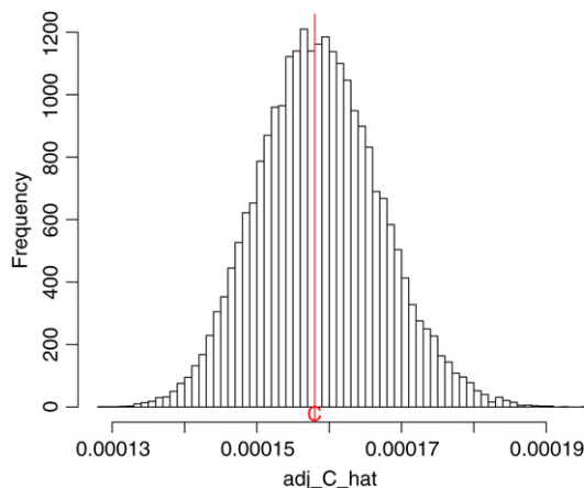
Fig. 3. Histogram of \hat{C}_t^{n,\text{adj}} , for Model 1.
