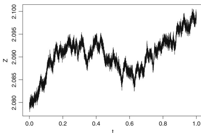
Fig. 1. One observed sample path generated by model 1.
