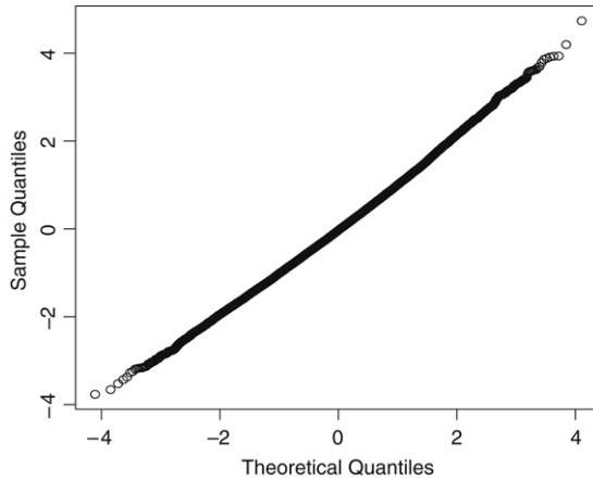
Fig. 5. Normal Q – Q plot of N0_t^{n,\text{adj}} for Model 1.
