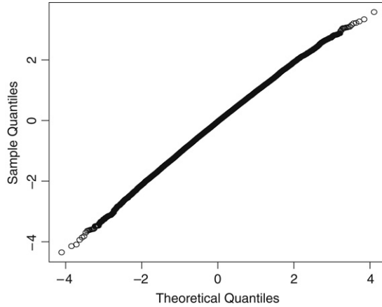
Fig. 4. Normal Q – Q plot of N_t^{n,\text{adj}} for Model 1.
