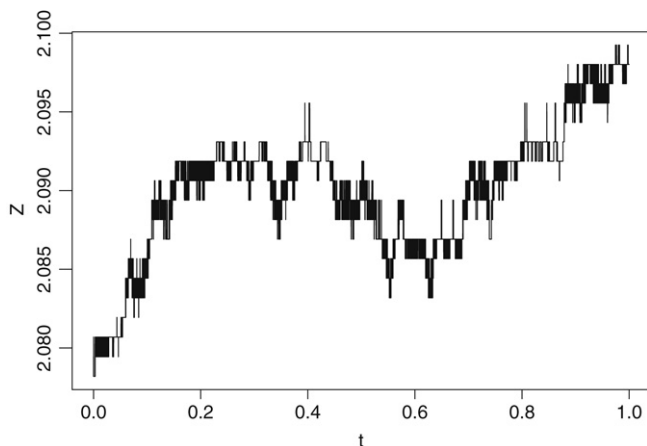
Fig. 2. One observed sample path generated by model 2.
