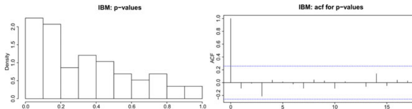
FIGURE 4. Histogram and ACF plot of the daily p -values for IBM 2005 Jan-Mar three-months data.
