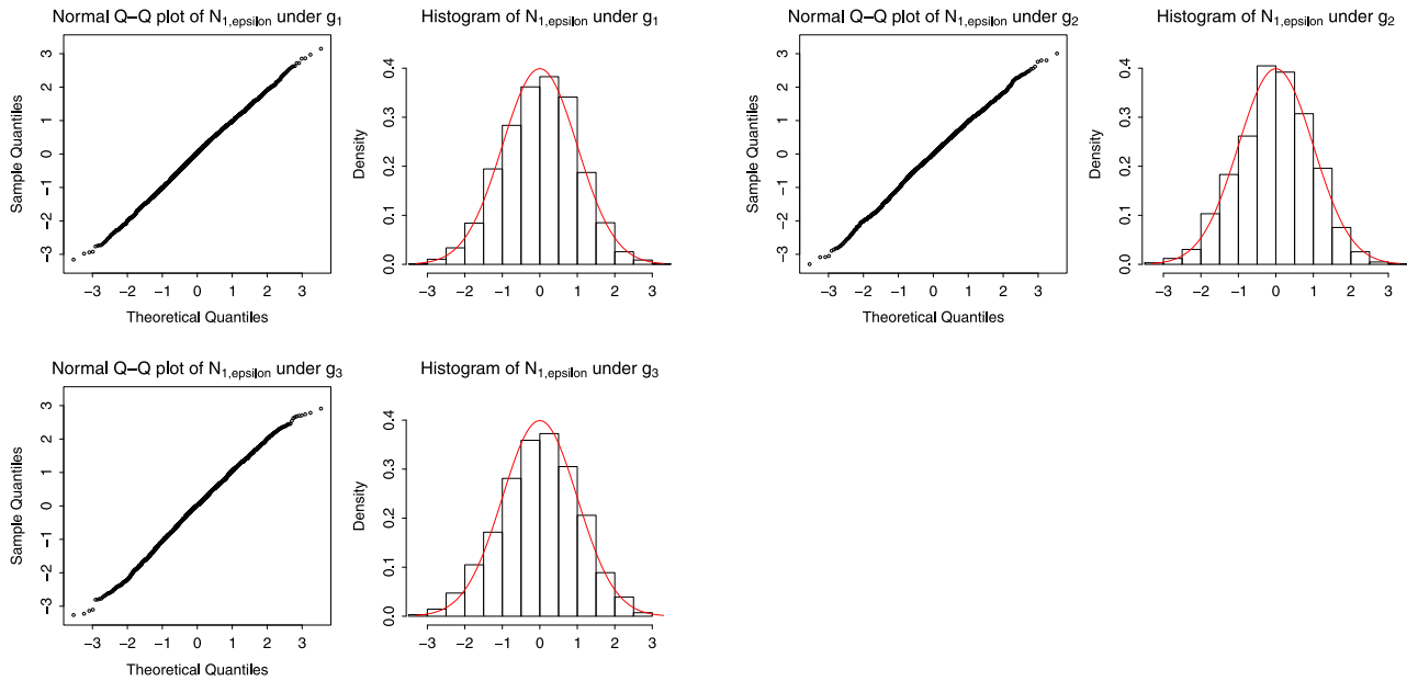
Fig. 1. Normal Q–Q plot and histogram based on 2500 replications of N_{1,\epsilon}^n under model (36) with X satisfying (35), and g being g_1 (upper-left), g_2 (upper-right) and g_3 (lower), for the Poisson arrival time case. In each of histogram, the red curve is the density plot of the standard normal distribution. (For interpretation of the references to color in this figure legend, the reader is referred to the web version of this article.)
