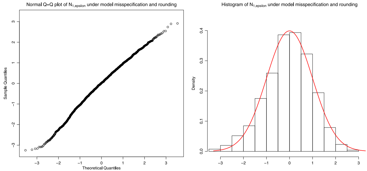
Fig. 2. Normal Q–Q plot and histogram of N_{1,\epsilon}^n under model misspecification and rounding in both price and time. The red curve in the histogram is the density plot of the standard normal distribution. (For interpretation of the references to color in this figure legend, the reader is referred to the web version of this article.)
